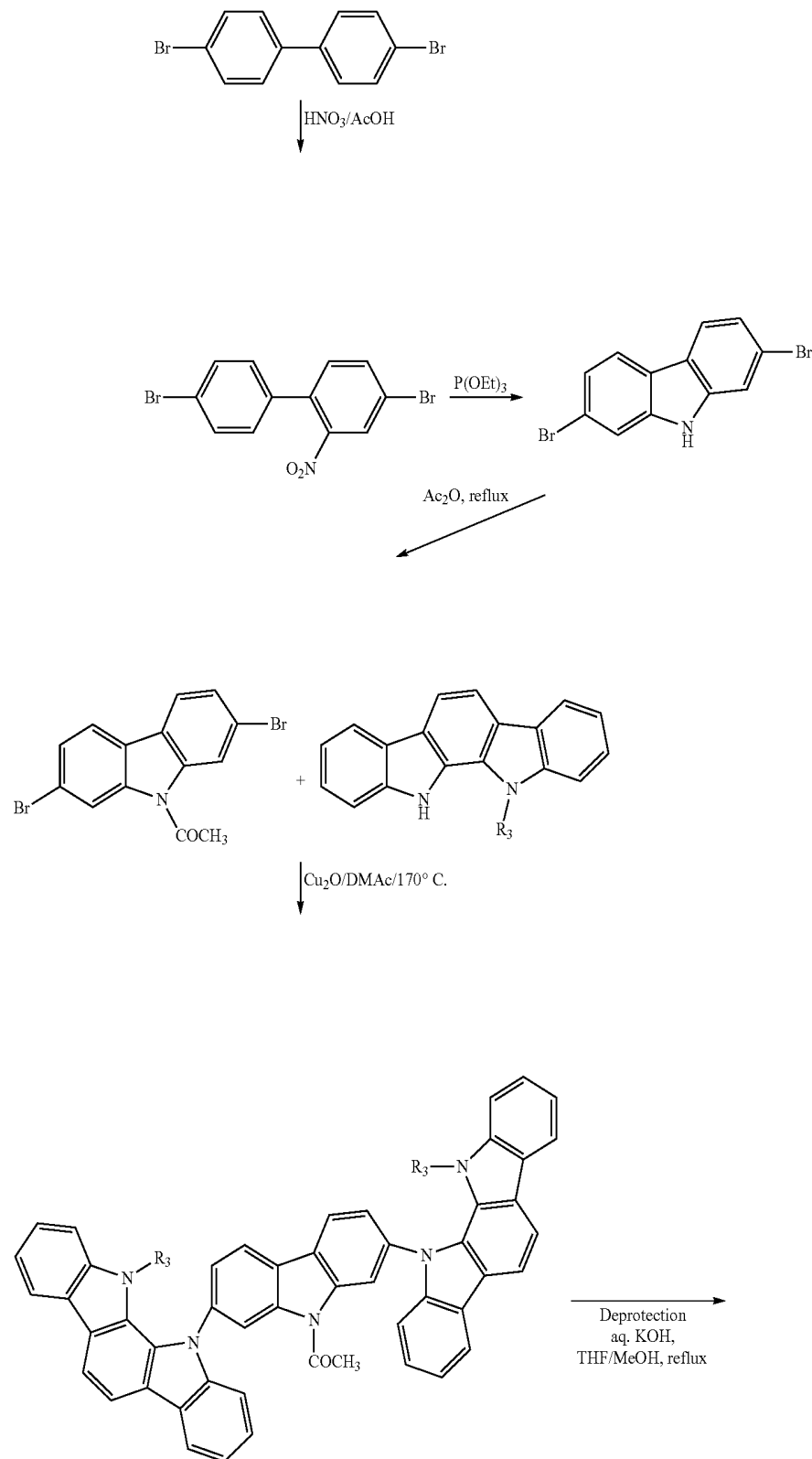
Scheme 6: Synthesis of compounds from 4-6 to 4-9
