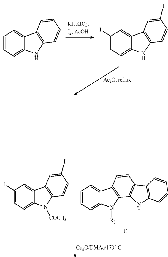
Scheme 3: Synthesis of compounds from 3-1 to 3-7
