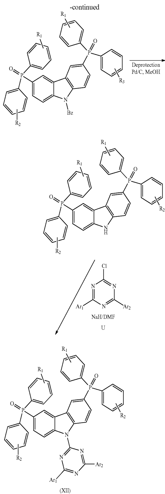
Scheme 12: Synthesis of compounds from 8-8 to 8-12
