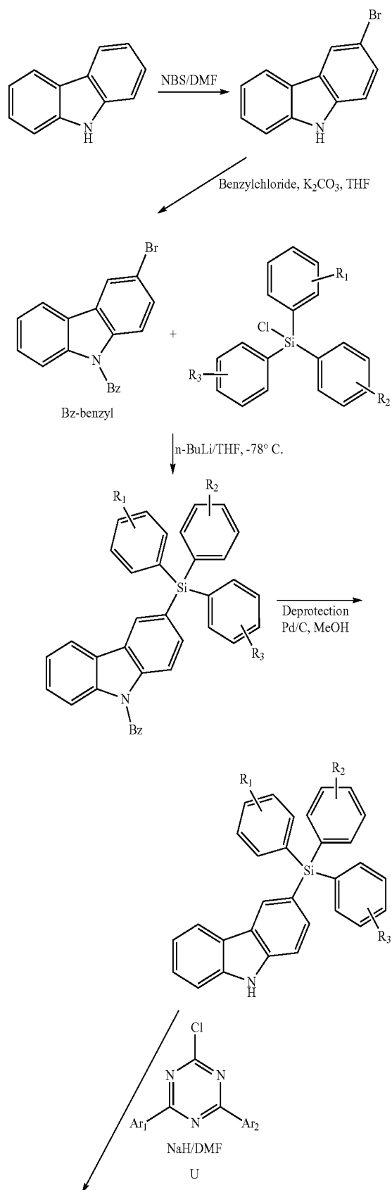
Scheme 10: Synthesis of compounds from 7-6 to 7-10
