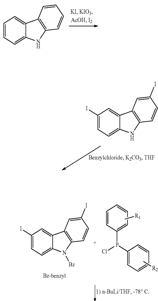
Scheme 11: Synthesis of compounds from 8-1 to 8-7
