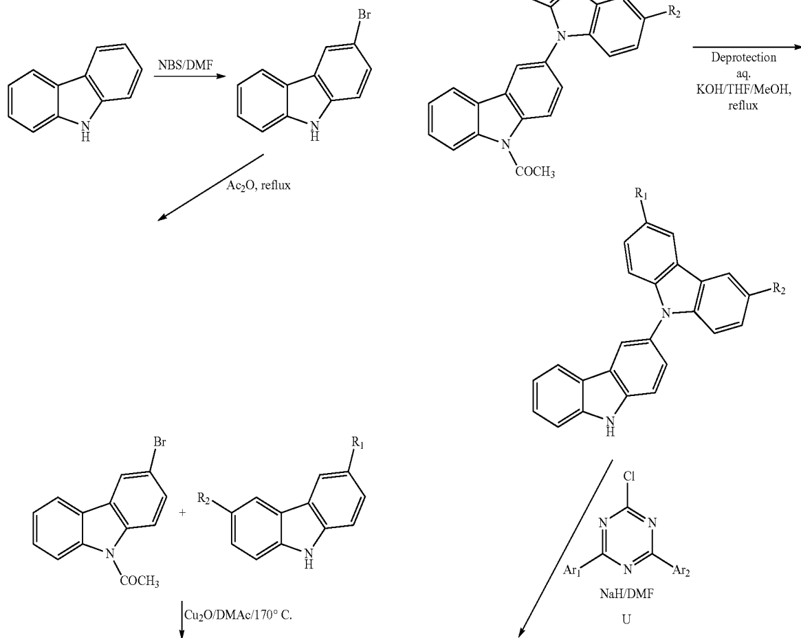
Scheme 2: Synthesis of compounds from 2-1 to 2-10
