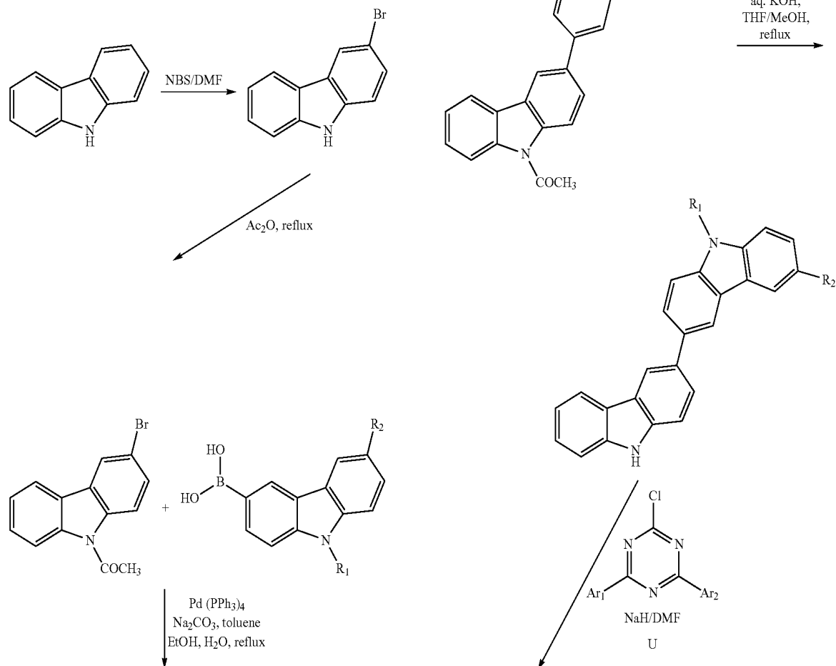
Scheme 8: Synthesis of compounds from 6-1 to 6-6
