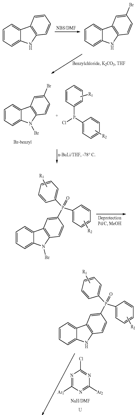
Scheme 12: Synthesis of compounds from 8-8 to 8-12
