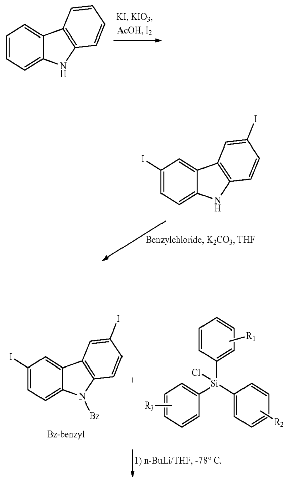
Scheme 9: Synthesis of compounds from 7-1 to 7-5
